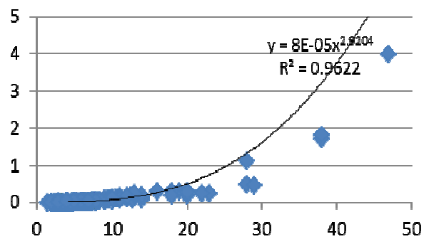
Fig.9. Forest productivity for Sessile oak forest type
