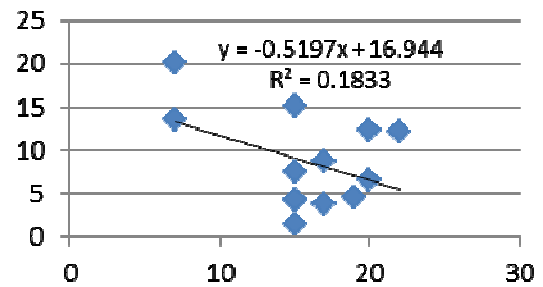
Fig.10. Forest increment per age, for Turkey, Hungarian oak forest type
