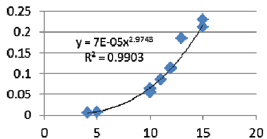
Fig.11. Forest productivity per diameter, for Turkey, Hungarian oak forest type
