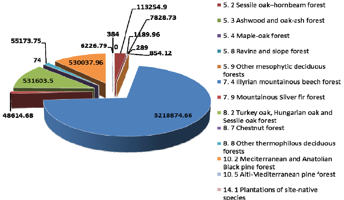
Fig.6. The structure of forest types for volume
