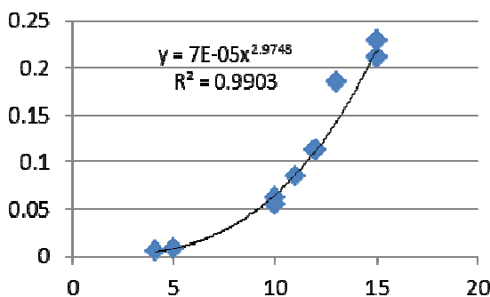
Fig.14. Forest productivity for introduced tree species
