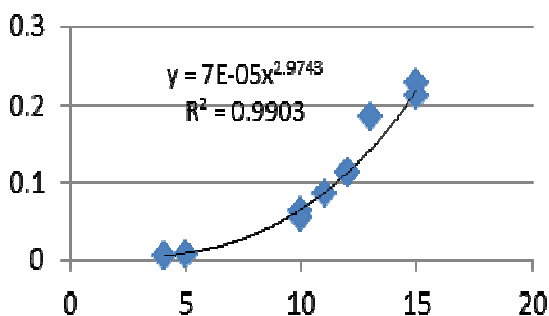
Fig.13. Forest productivity for Black pine forest type
