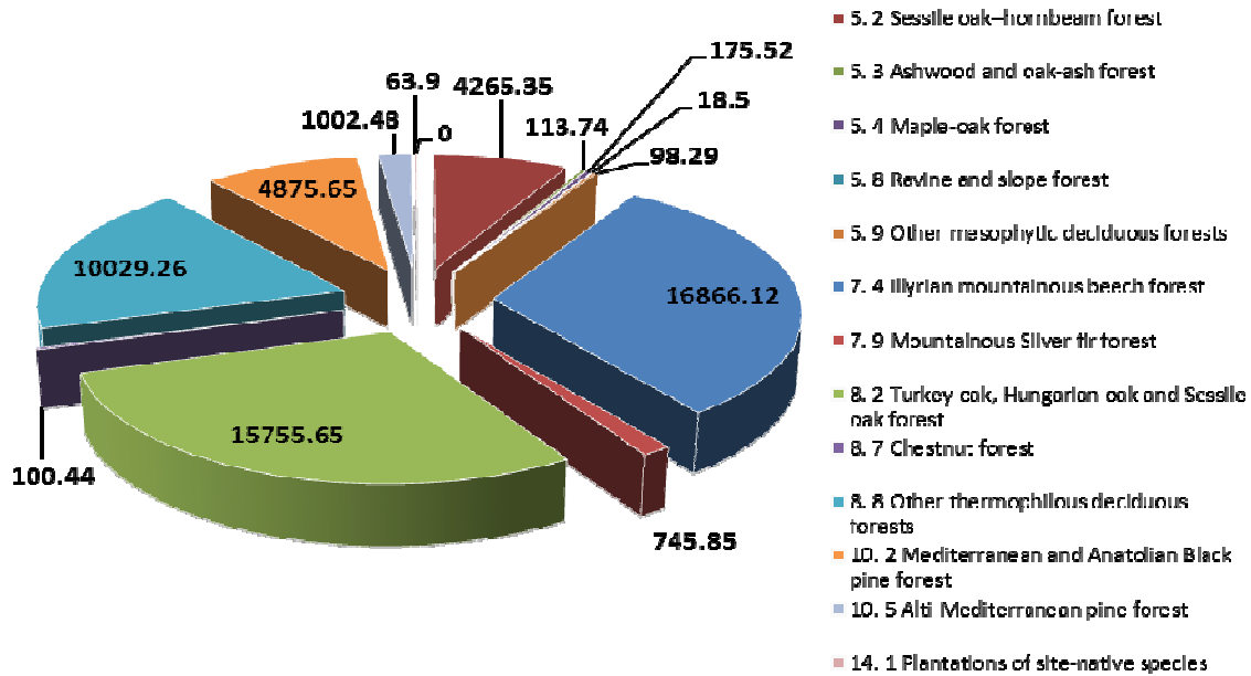
Fig.5. The structure of forest types for area
