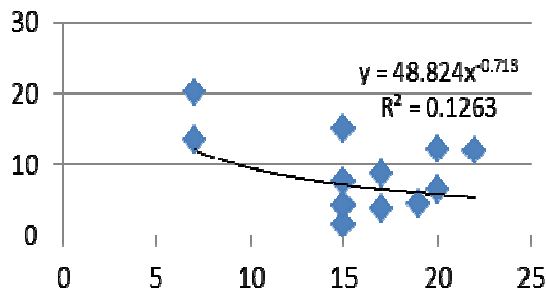
Fig.12. Forest increment for Black pine forest type
