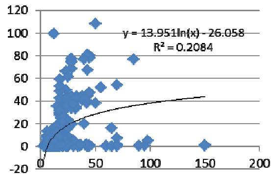
Fig.8. Forest increment per age, for Sessile oak forest type
