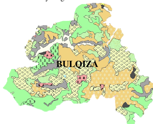
Fig.3. Map of Forest types of Bulqiza's District
