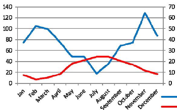
Fig.2. Gaussen aridity index of Bulqiza region
