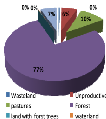
Fig.4. Land use of Bulqiza's region
