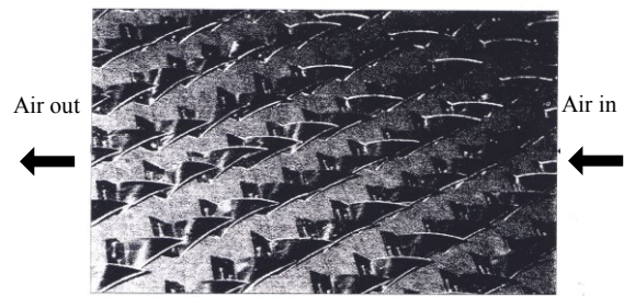
Photograph 2 : Layout with OCL1 type baffles
