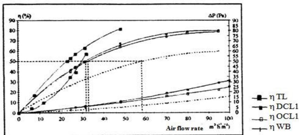
Figure. 6: Evolution of thermal efficiency (where I_{GS} = 1063.5W/m^2 ) and charge losses in relation to air flow as concerns WB solar panels and those provided with different types of baffles ( i.e. DCL1, OCL1 and then TL), as at the Valenciennes site
