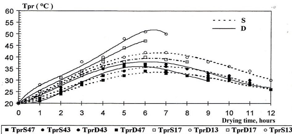
Figure 10: Evolution of the temperature of girolle mushroom in relation to drying time measured at the first and fourth trays with flows of 31.3\text{m}^3/\text{h.m}^2 and 70\text{m}^3/\text{h.m}^2 using WB, DCL1 and TL type solar panels
