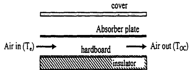
Figure 2. Solar air flat plate collector without obstacles
