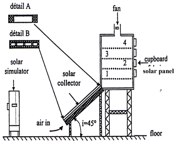
Figure 1. Experimental device
