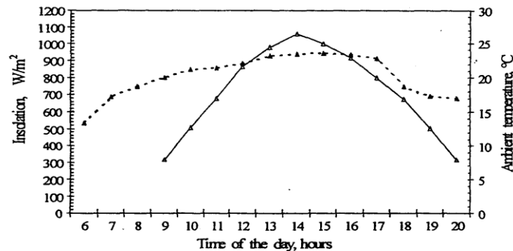
Figure 3. Variation of the ambient temperature and the insolation during the characteristic day of July, at Valenciennes — \Delta — global hourly insolation ( I_{gh} ); — \square — ambient temperature ( T_a )
