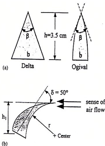
Figure 5: Diagram of delta and ogival obstacles (a) before the waisting (b) after the waisting
