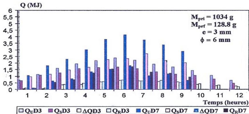
Figure. 13: Variations in quantities of heat (Q) in relation to drying time with flows of 31.3m 3 /h.m 2 and 70m 3 /h.m 2 using a solar panel equipped with DCL1 baffles
