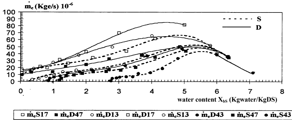
Figure. 11: Evolution of the drying speed ( m_c ) in relation to water content to the point when the product is completely dried with flows of 31.3\text{m}^3/\text{h.m}^2 and 70\text{m}^3/\text{h.m}^2 using WB and DCL1 type solar panels
