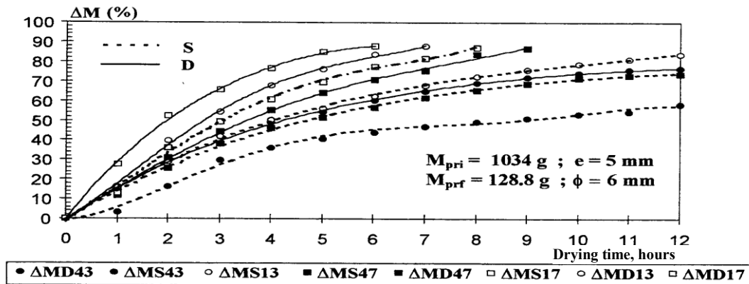
Figure 9: Evolution of the loss of mass ( \Delta M ) of plums in relation to drying time measured at the first and fourth trays with flows of 31.3\text{m}^3/\text{h.m}^2 and 70\text{m}^3/\text{h.m}^2 using DCL1 and TL type solar panels, data recorded on a typical July day at the Valenciennes site
