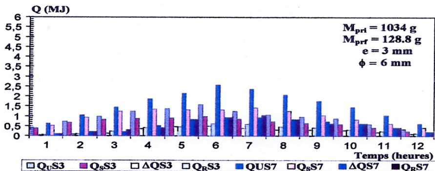
Figure. 12: Variations in quantities of heat ( Q ) in relation to drying time with flows of 31.3\text{m}^3/\text{h.m}^2 and 70\text{m}^3/\text{h.m}^2 using an WB type solar panel (without baffles)
