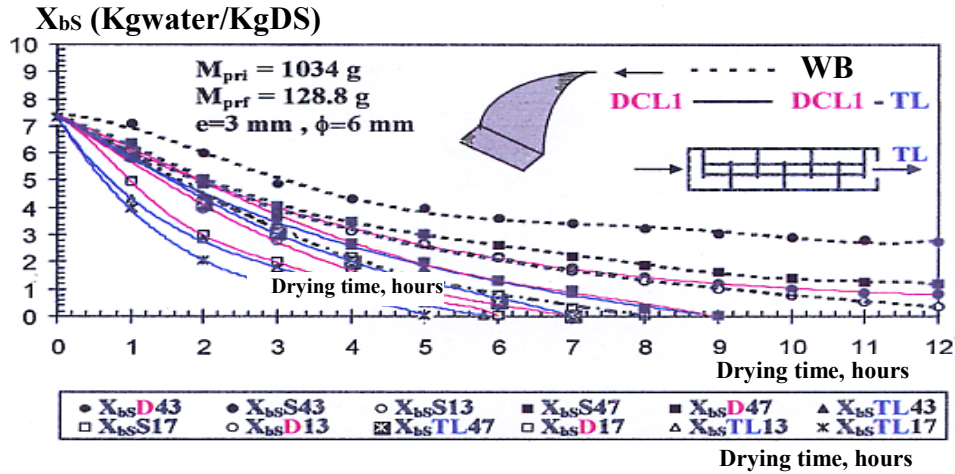
Figure 8: Evolution of the water content ( X_{bs} ) in relation to drying time measured at the first and fourth trays with flows of 31.3\text{m}^3/\text{h.m}^2 and 70\text{m}^3/\text{h.m}^2 using WB, DCL1 and TL type solar panels, data recorded on a typical July day at the Valenciennes site
