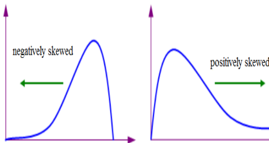
Fig. 1. positively and negatively skewed
