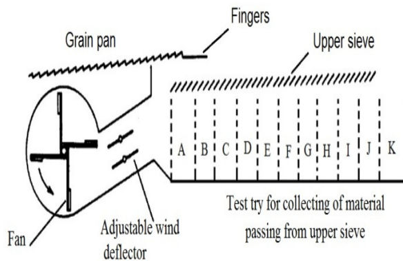
Fig 3. A schematic diagram of a cleaning mechanism
