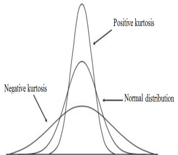
Fig. 2. Positive and negative kurtosis and normal distribution
