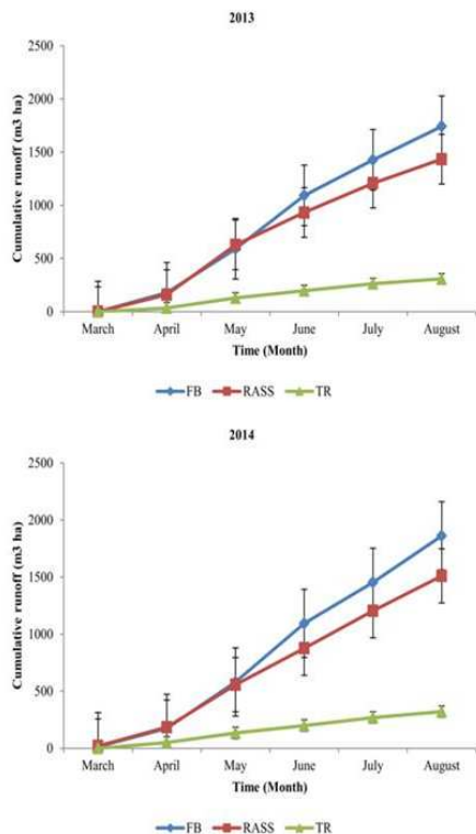
Fig. 5. Chart of average cumulative runoff per hectare, per tillage method on 29% slope
