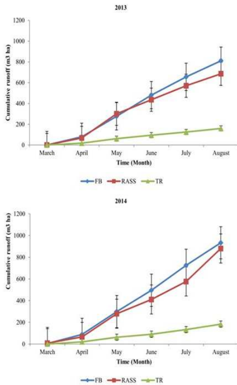
Fig. 4. Chart of average cumulative runoff per hectare, per tillage method on 11% slope
