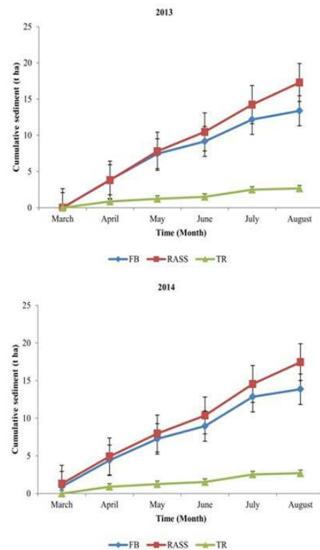
Fig. 6. Chart of average cumulative sediment per hectare, per tillage method on 11% slope
